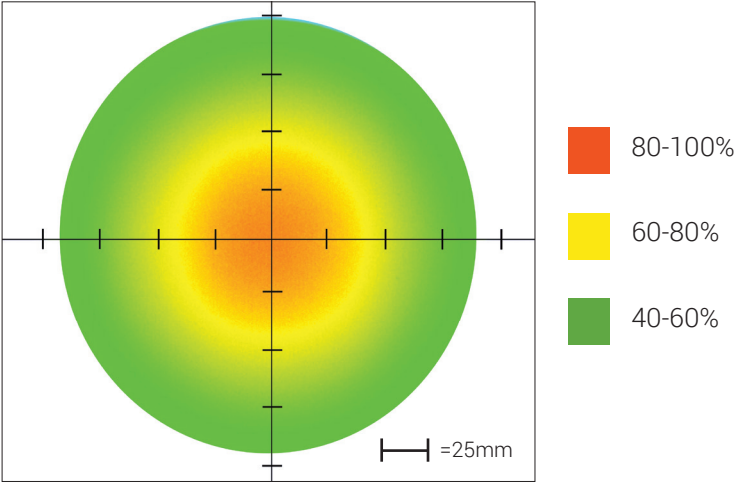
Optical measurement taken using RL127-WHIC @ 200 mm
